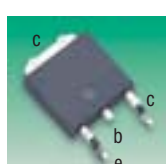
(c) TO-252/D-pak H=2.55, W=6.8, D=10.5
