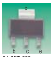
(b) SOT-223 H=1.7, W=6.7, D=7.3
