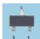
(a) SOT-23 H=1.12, W=3.05, D=2.5
